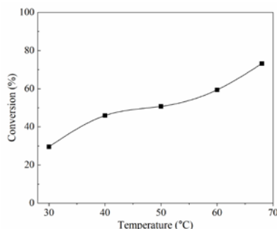
Figure 6. Effect of reaction temperature (CS-RH-900, time: 7 h, catalyst loading: 10 wt%, molar ratio of MeOH/oleic acid: 10:1)
