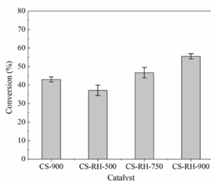
Figure 4. Effect of catalyst type
