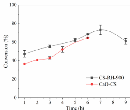
Figure 5. Effect of reaction time
