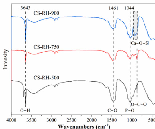
Figure 3. FT-IR spectra of CS-RH catalysts at different calcination temperatures
