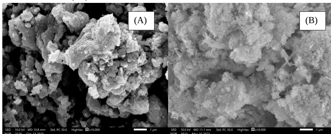
Figure 1. SEM Images of (A) CaO From Crab Shells and (B) CS-RH CaO-SiO 2
