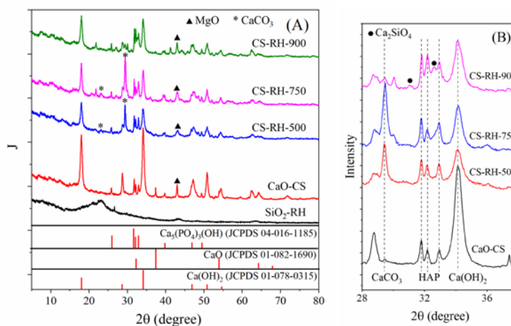
Figure 2. XRD patterns of CS-RH catalyst at different calcination temperatures: (A) full 2θ range, (B) narrow 2θ range
