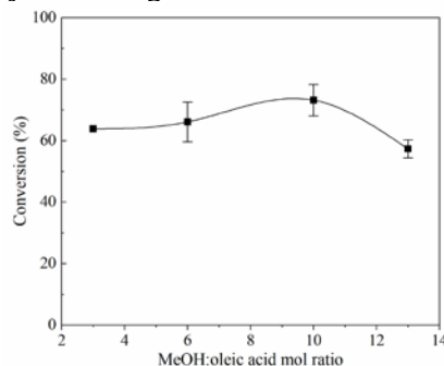
Figure 7. Effect of molar ratio of MeOH/oleic acid (CS-RH-900, temperature: 68 °C, time: 7 h, catalyst loading: 10 wt%)
