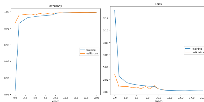
Figure 3. Training Results Using the Dataset Preprocessed According to the Proposed Method
