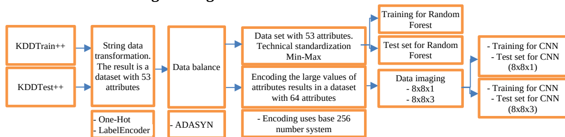
Figure 1. Data preprocessing process
